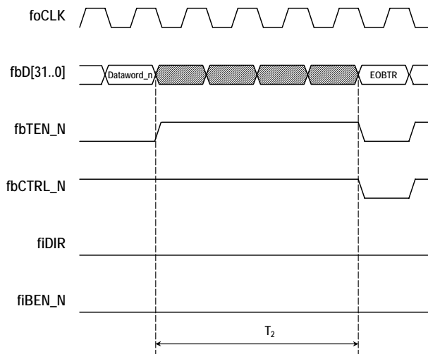
Figure 14 The end of a data block write transaction
