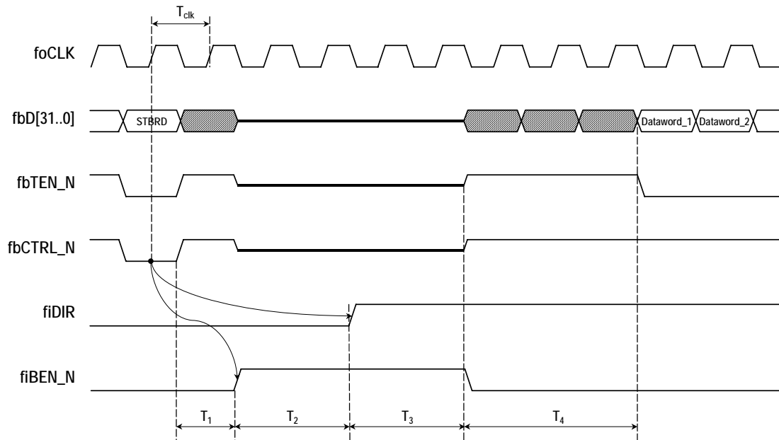
Figure 15 The opening of a new data block read transaction
