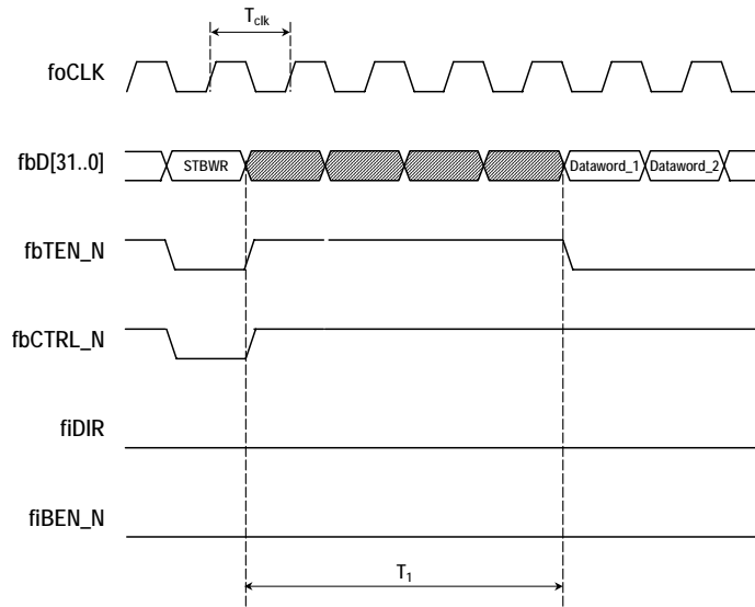
Figure 13 The opening of a data block write transaction
