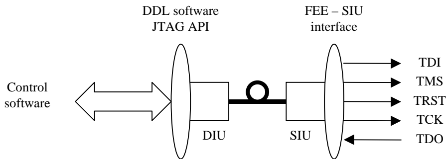
Figure 22 Basic structure of the JTAG chain.
