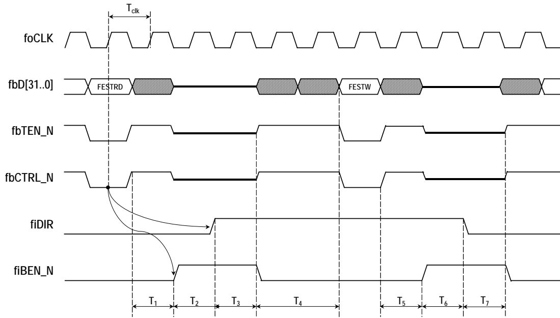
Figure 12 The front-end status read-out transaction
