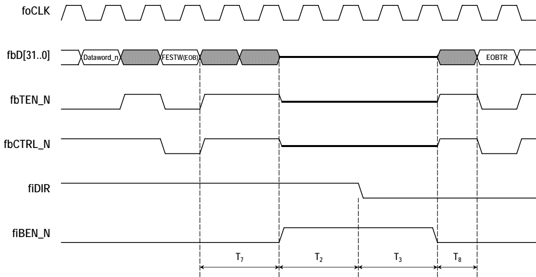
Figure 19 The end of an event data transmission transaction
