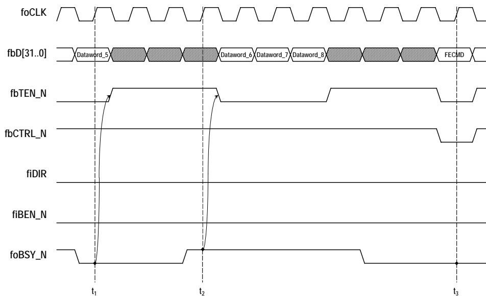
Figure 20 The flow-control for the data transfer from the SIU to the FEE
