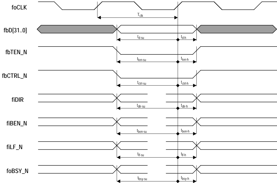
Figure 9 Timing waveforms of the FEE-SIU interface signals
