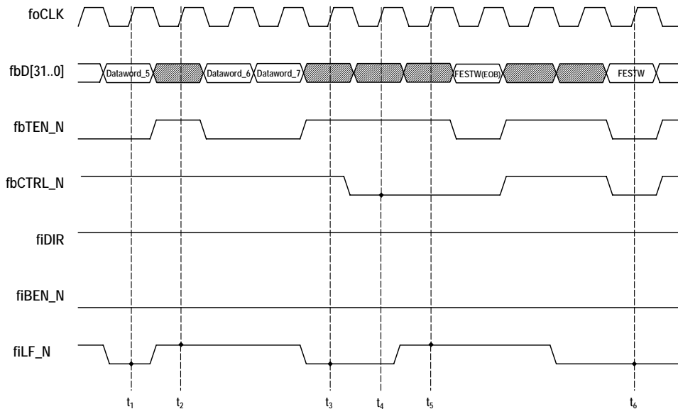
Figure 21 The flow-control for the data and status transfer from the FEE to the SIU
