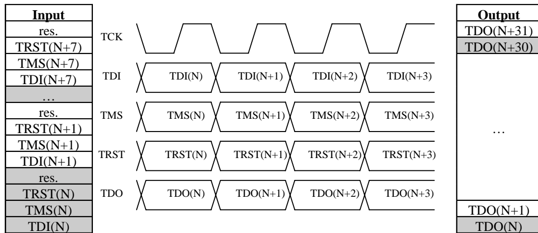
Figure 23 Example of the JTAG operation
