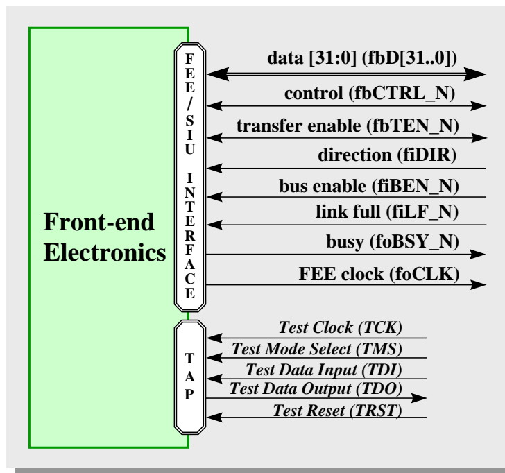
Figure 5 The names of the SIU-FEE interface and the TAP signals
