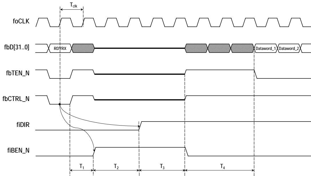
Figure 17 The opening a new event data transmission transaction
