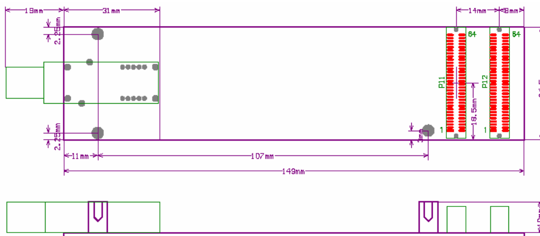
Figure 3 The physical arrangement of the SIU card
