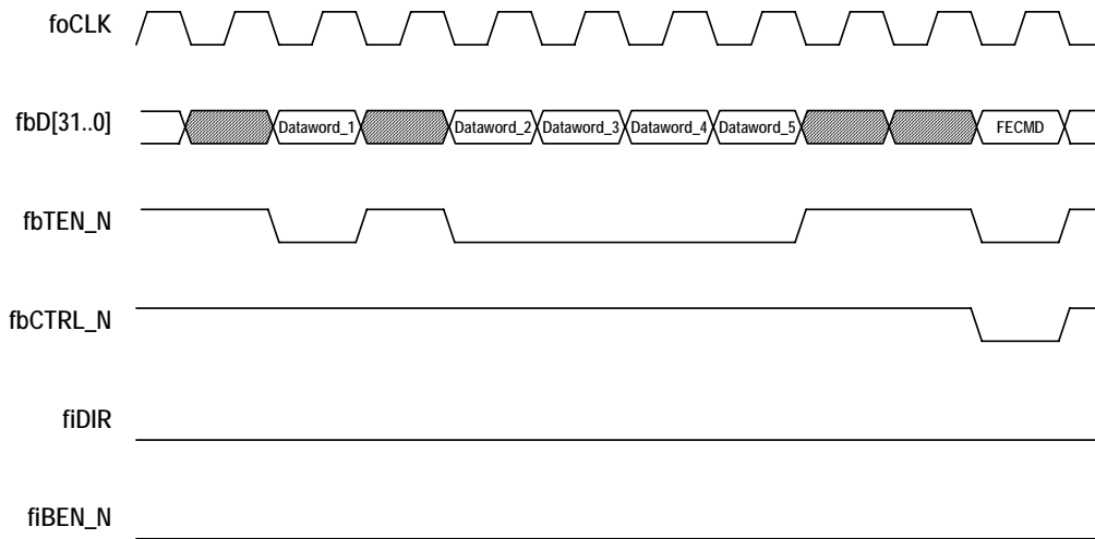
Figure 10 Data and command transfer from the SIU to the FEE
