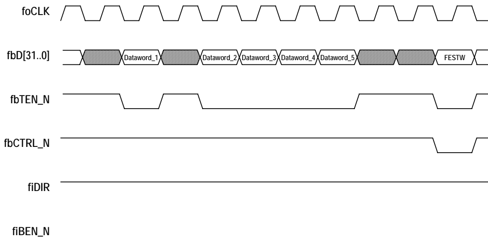
Figure 11 Data and status word transfer from the FEE to the SIU
