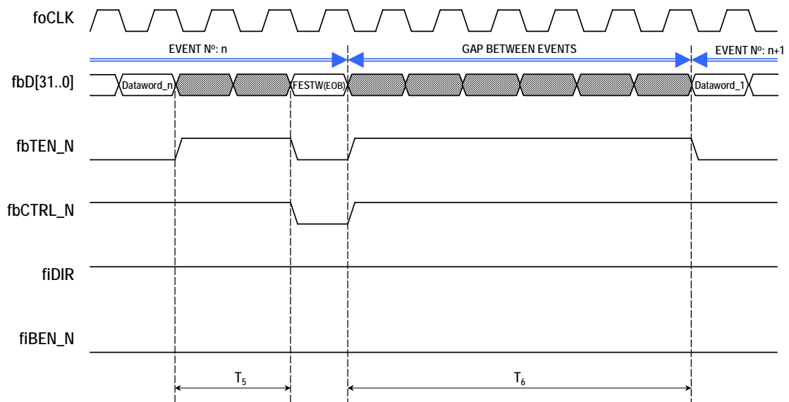
Figure 18 The end of an event transmission and the start of a new event transmission
