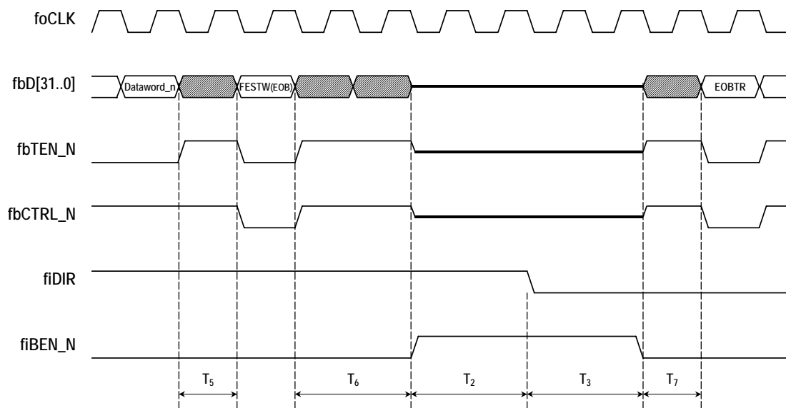
Figure 16 The end of a data block read transaction
