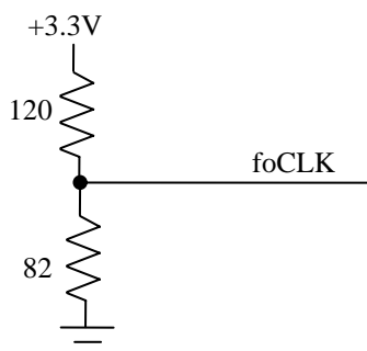
Figure 4 The resistive termination on the foCLK input signal
